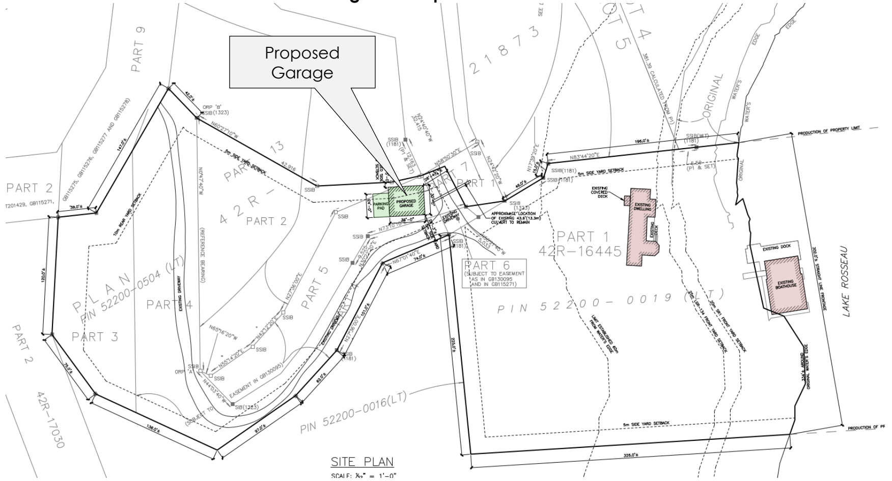
Figure 2: Proposed Site Plan
